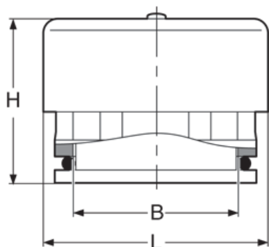
Anti pressure vent in PP-H, with a PE-HD yellow protection cap
